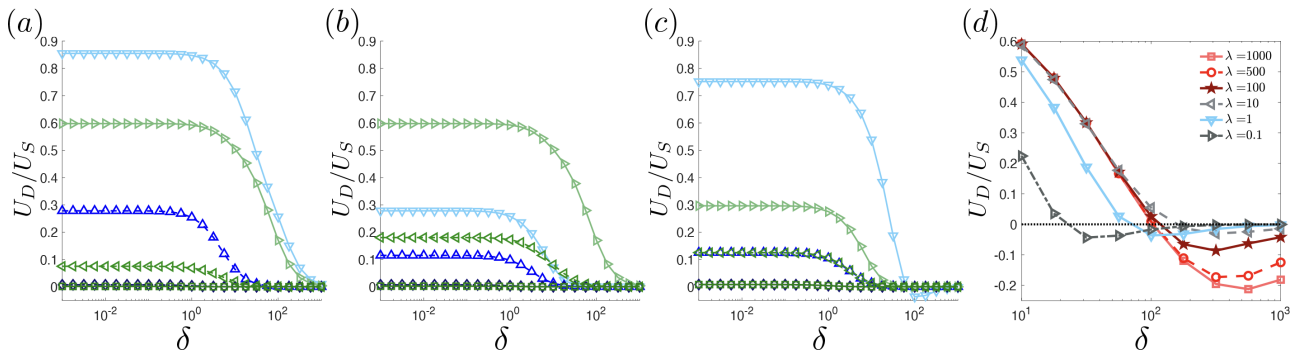
FIG. 4. Ratios of (a) the spherical droplet ( e_d=0 ) speed to the spheroidal squirmer speed, (b) the spheroidal droplet speed to the spheroidal squirmer speed, and (c) the spheroidal droplet speed to the spherical squirmer speed as a function of the fluid resistance with \lambda = 1 . Panels in (a)–(c) are color-coded to correspond to the squirmer’s speeds in Figs. 3(b), 3(e), and 3(h). In (d), the ratio is plotted for the spherical squirmer ( e_s=0 ) in a spheroidal droplet ( e_d=0.3 ). The panel shows changes in the range of fluid resistance and magnitude of the ratio that correspond to the backward propelling droplet ( U_D/U_S < 0 ). Each curve represents different values of the viscosity ratio \lambda .
